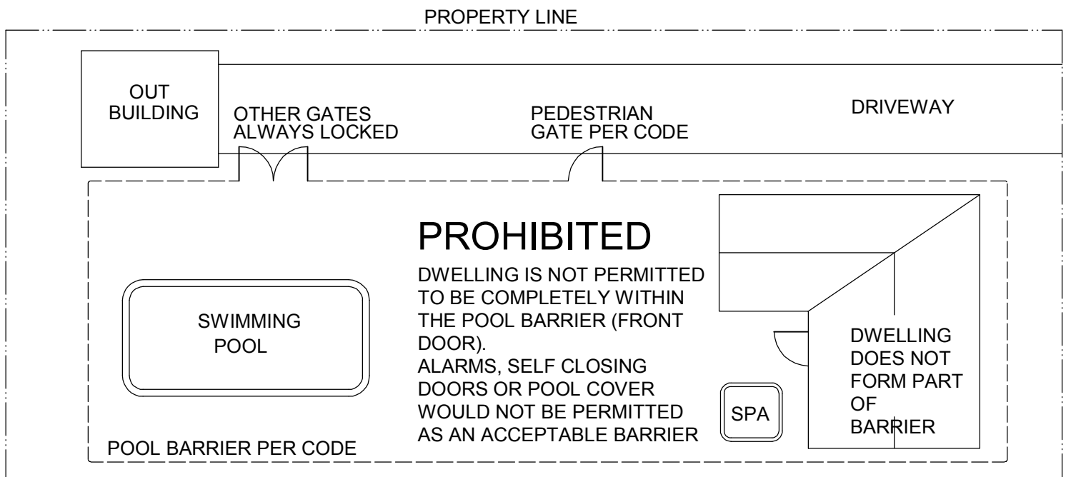
PLAN "D" - PROHIBITED LAYOUT
