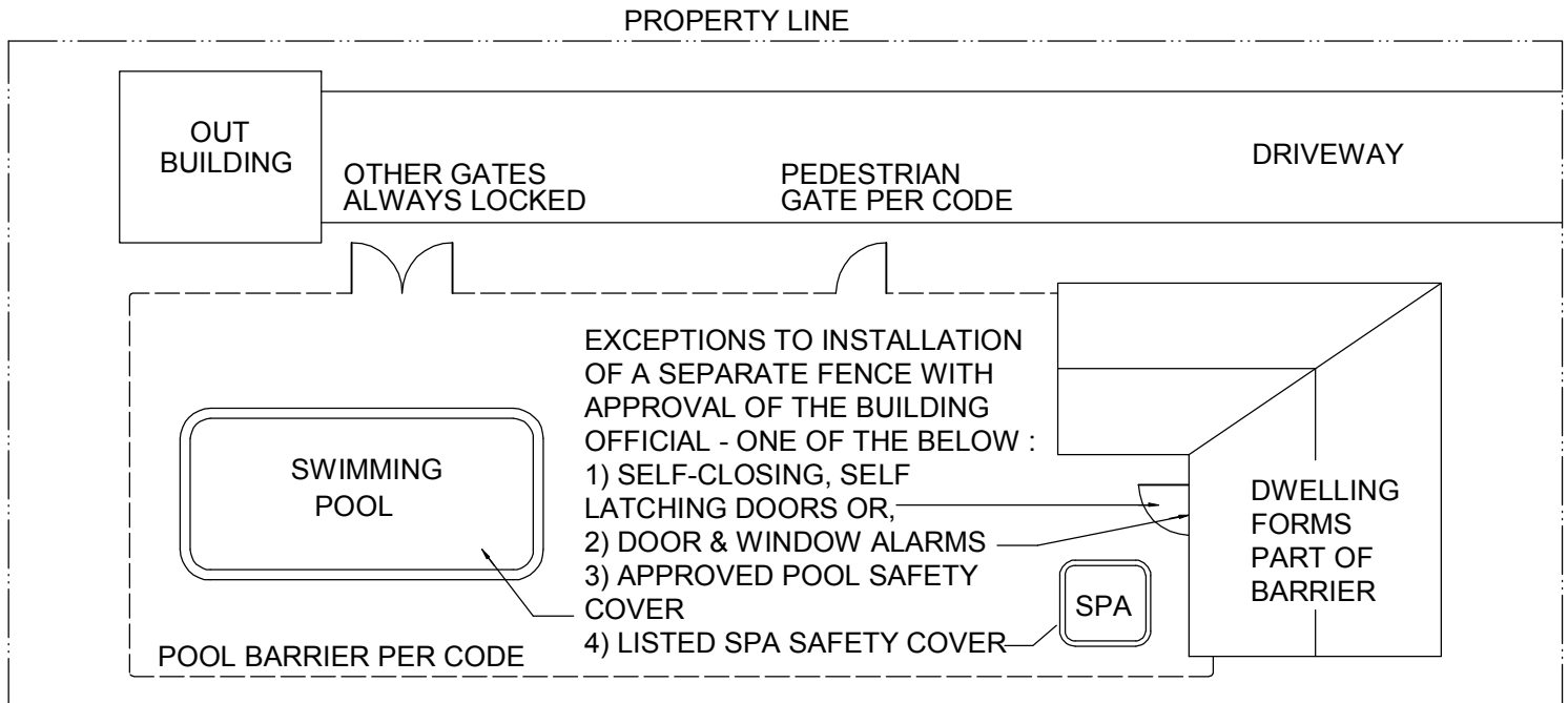
PLAN "C" - ACCEPTABLE LAYOUT WALL AS PART OF BARRIER
