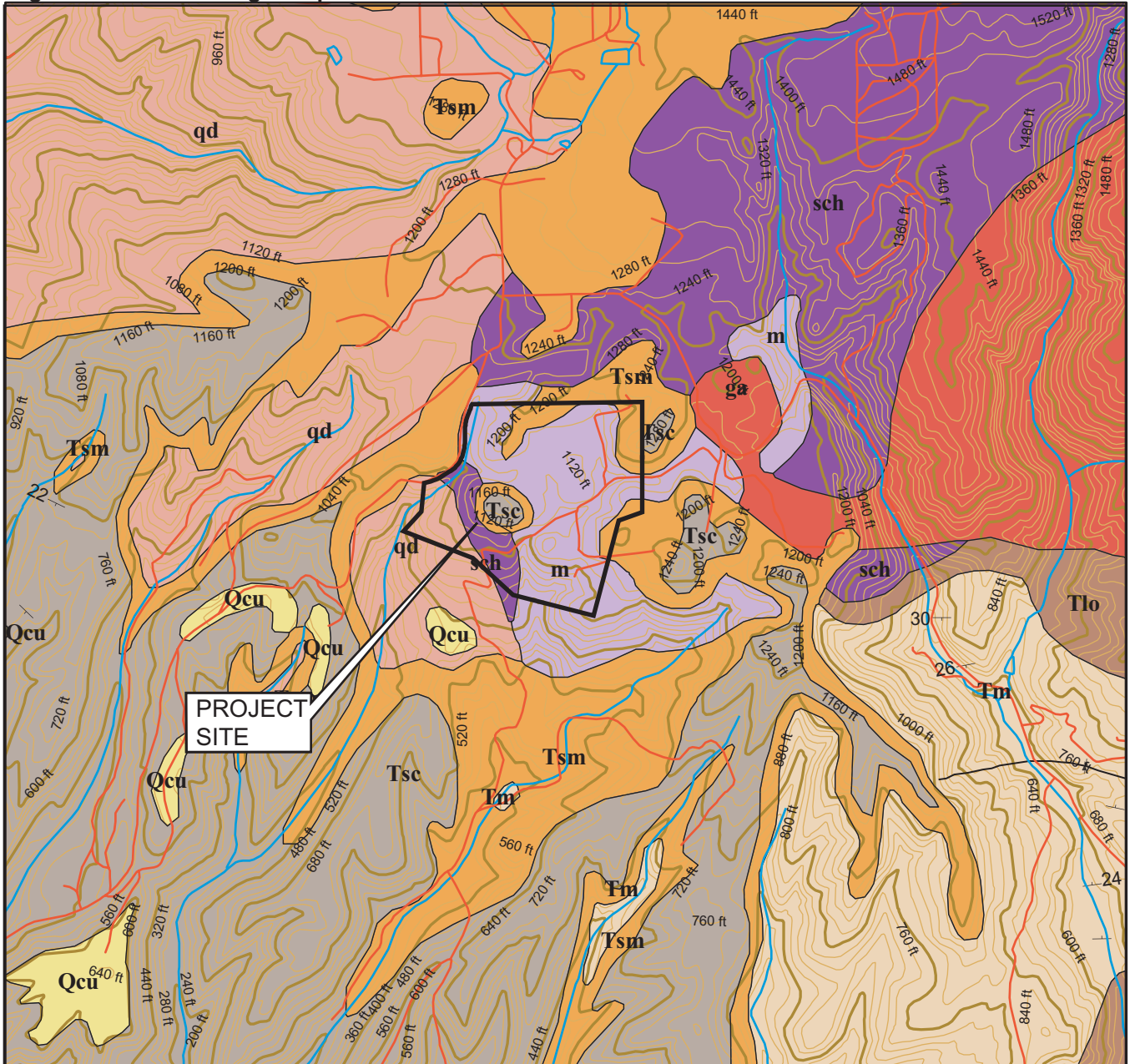
Figure 19. Local Geologic Map
