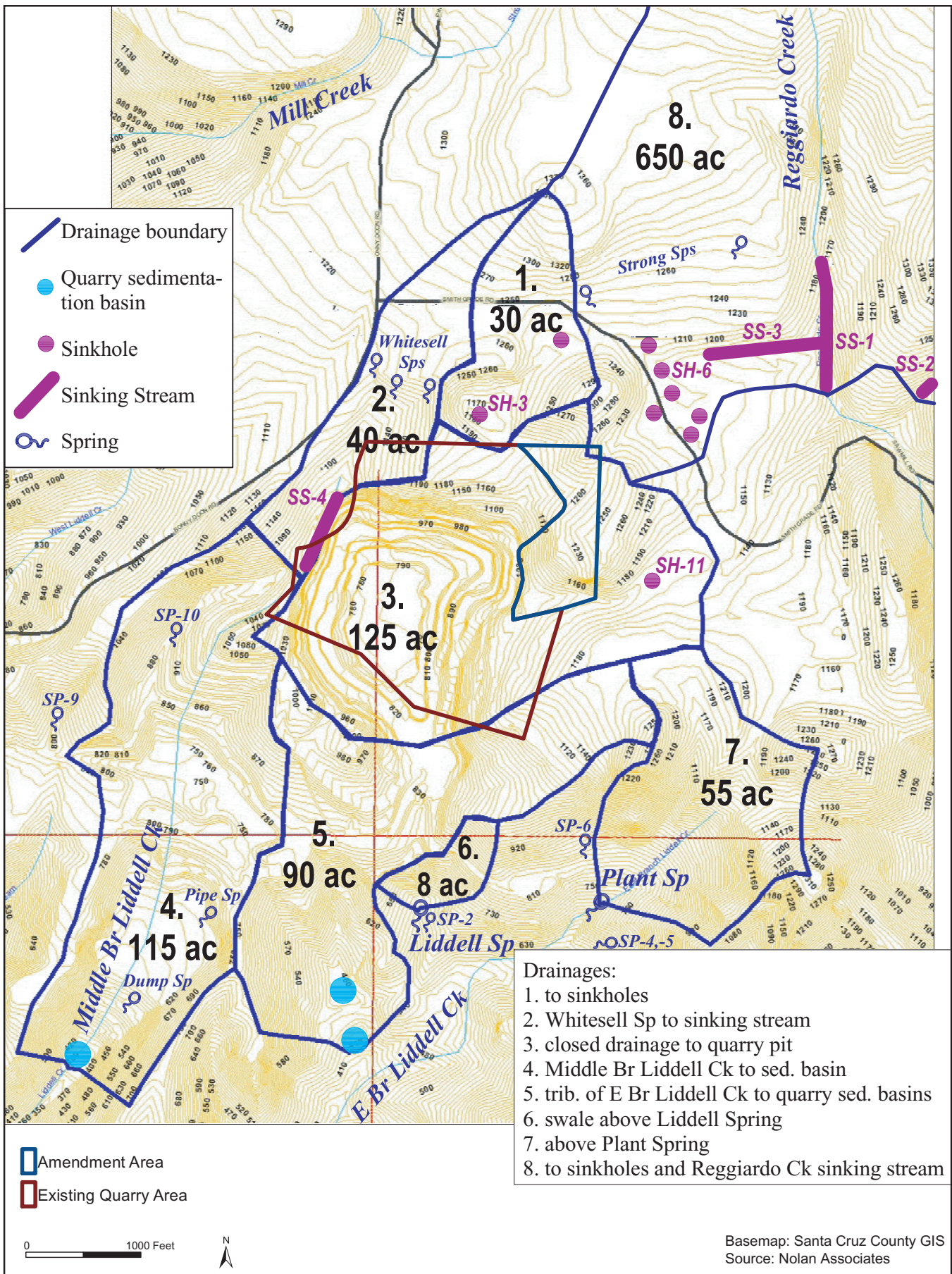
Figure 23. Approximate Quarry Area Drainages
