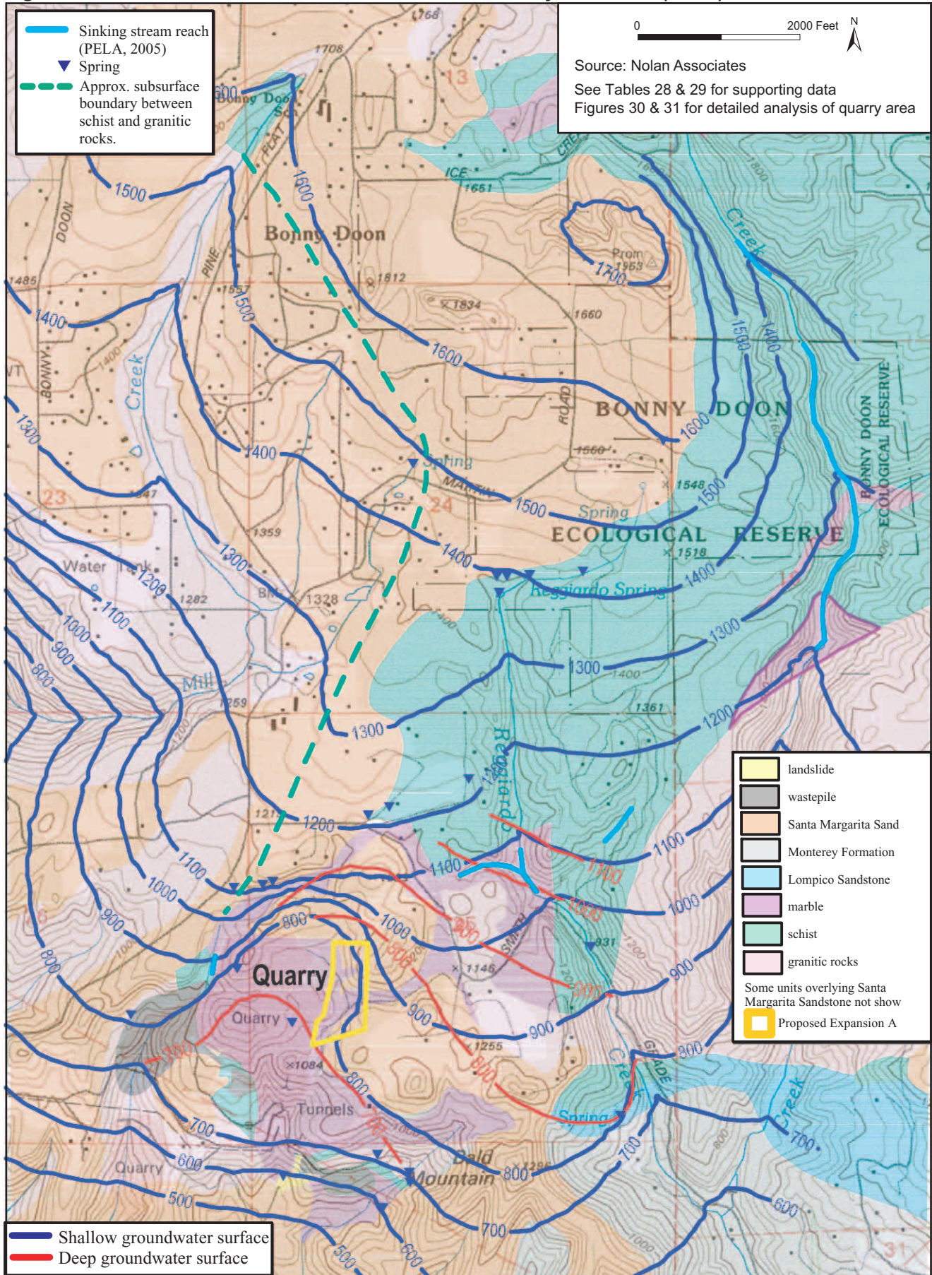
Figure 25. Generalized Groundwater Surface Contour, Bonny Doon Area (ft msl)
