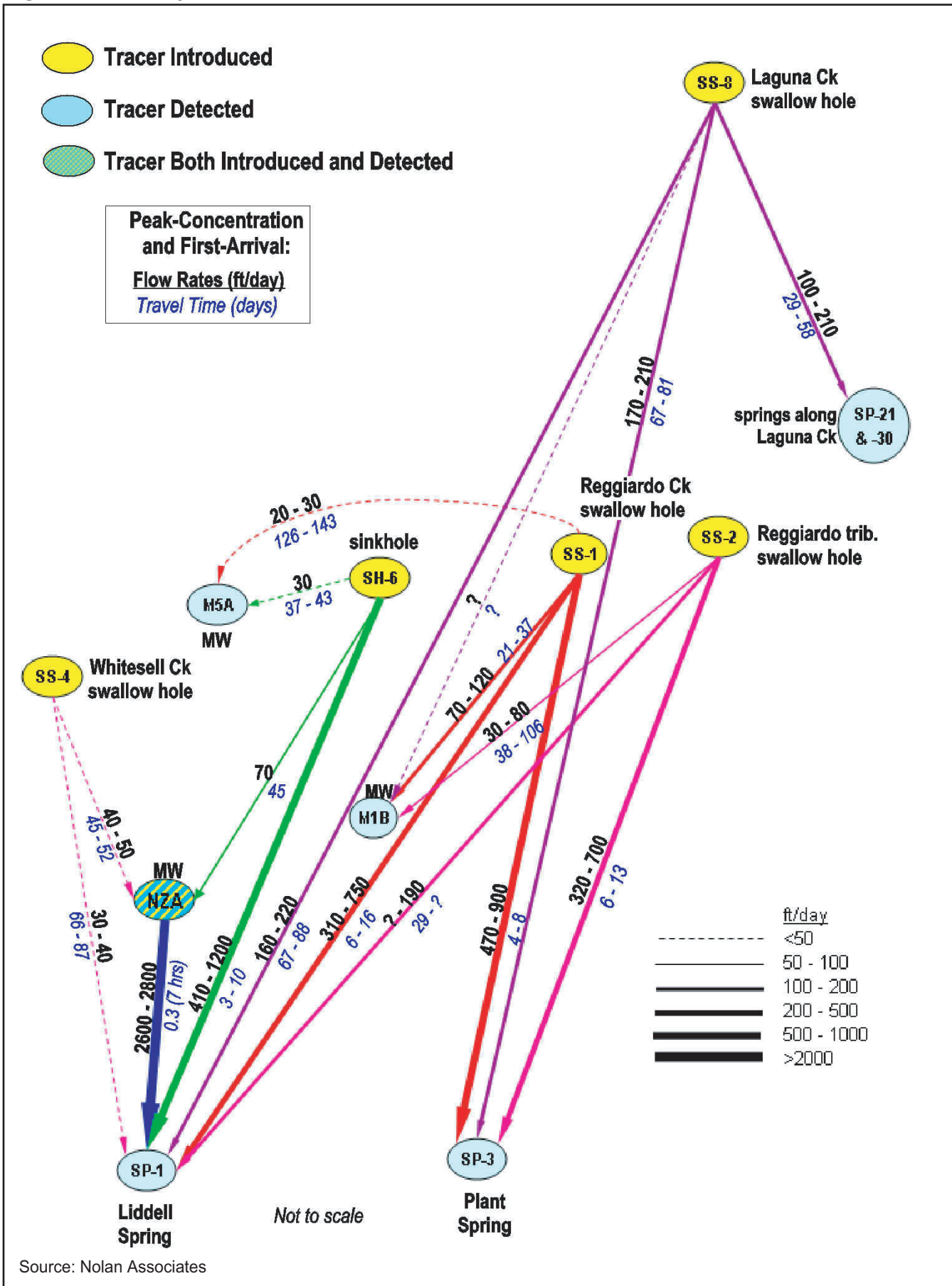
Figure 27. Summary of 2004 Tracer Test Results
