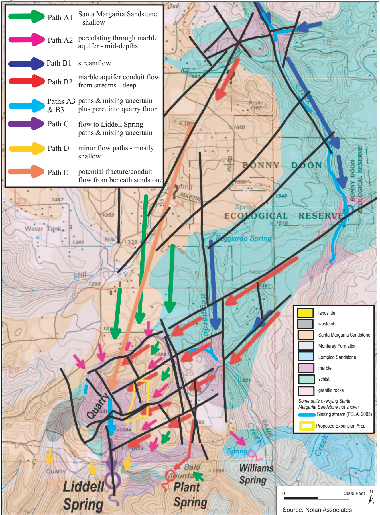
Figure 28. Principal Conceptual Groundwater Flow Paths
