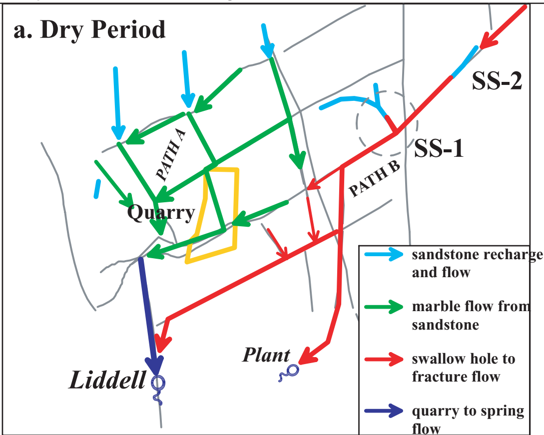
Figure 30. Conceptual Model of Seasonal Change in Groundwater Flow Pattern
