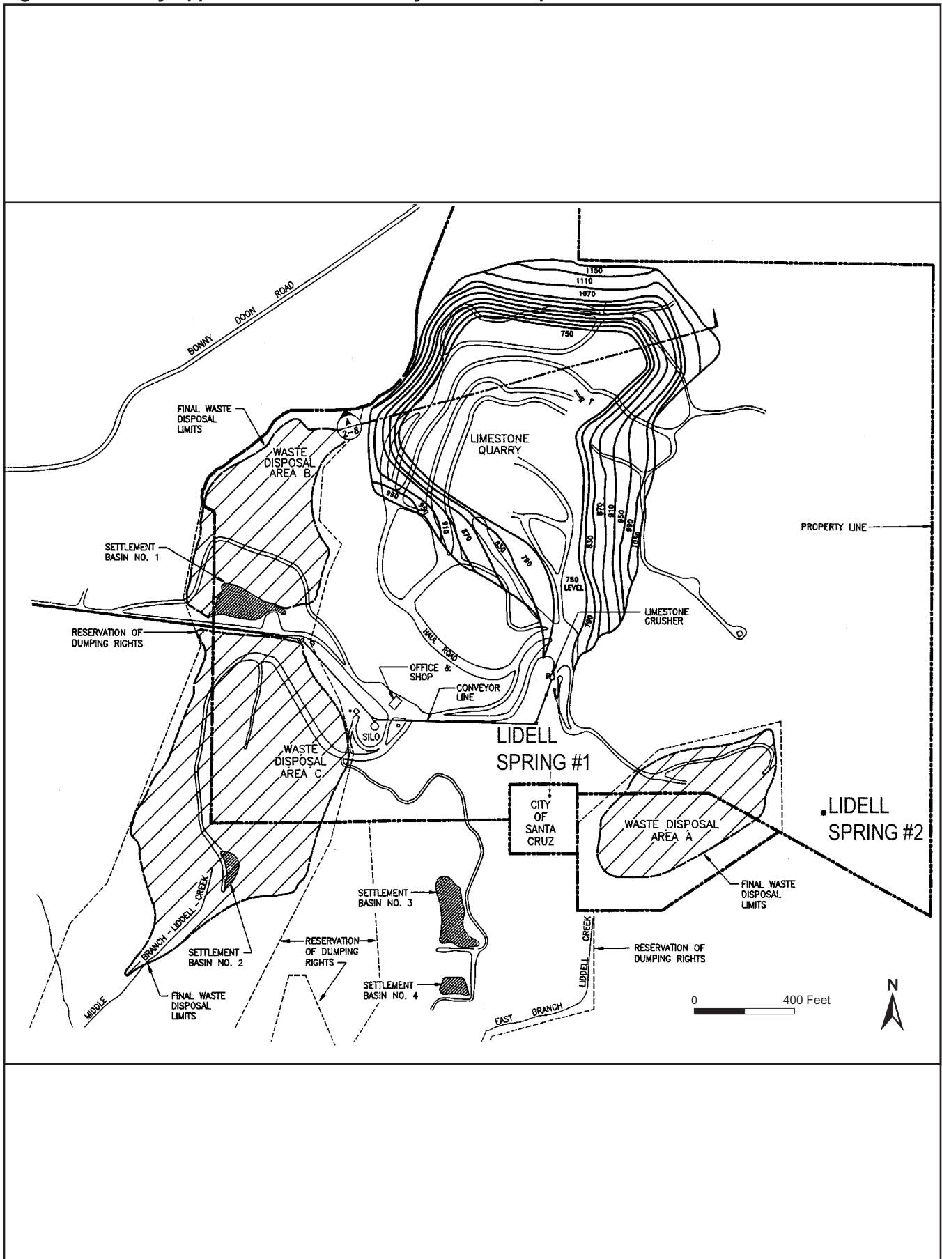
Figure 6. Currently Approved Limestone Quarry Final Development
